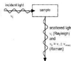
Figure 8.1: Scattering of light by a sample.
