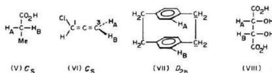
Figure 6.5 Enantiotopic ligands
