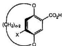
Chiral [n]cyclophane
