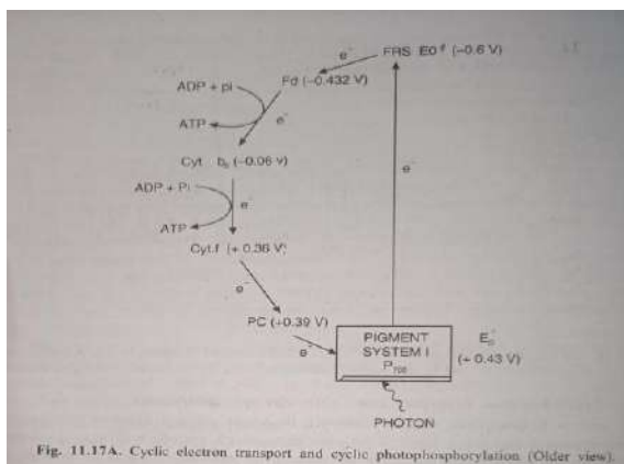
Fig. 11.17A. Cyclic electron transport and cyclic photophosphorylation (Older view).
