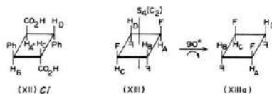
Figure 6.7 Enantiotopic ligands exchangeable through S_4 axis
