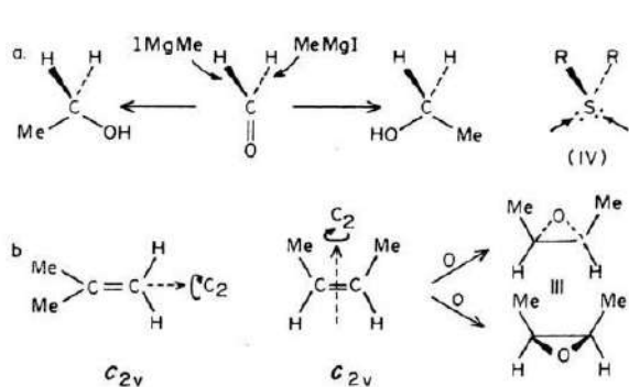
Figure 6.4 Homotopic faces
